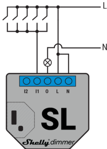
Momentary switch
