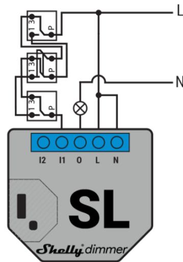
3-way switch
