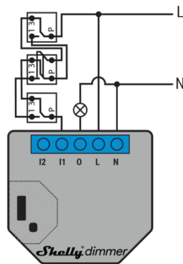
3-way switch
