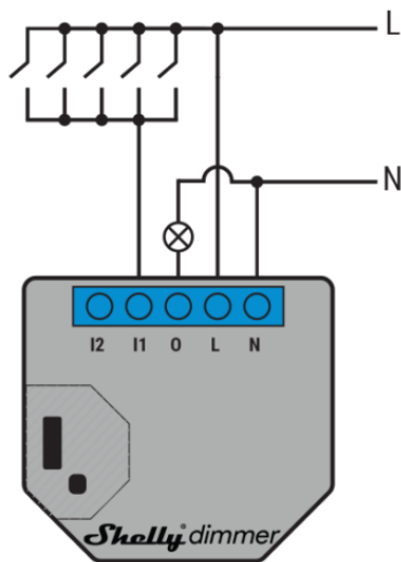
Momentary switch
